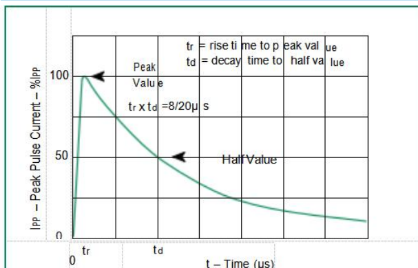
Figure 8 - Pulse Waveform
