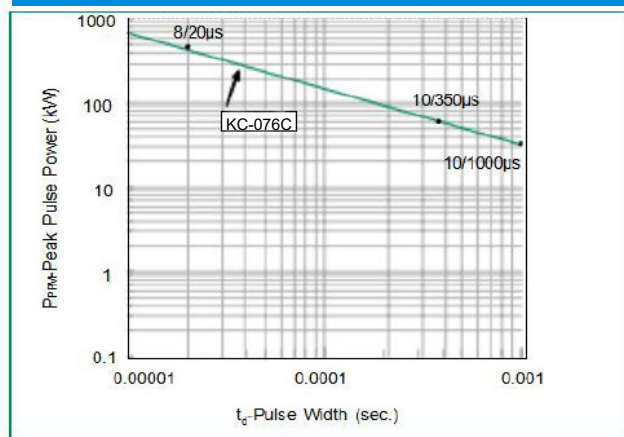
Figure 5 - Typical Peak Pulse Power Rating Curve
