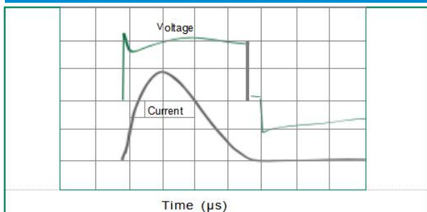
Figure 7 -Surge Response (8/20 Surge current waveform)
